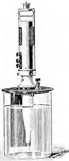
FIG. 21.—Single-point electrolytic interrupter. (Watson.)
